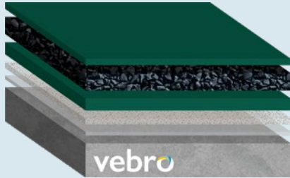
vebro Equestrian S A seamless, heavily cushioned polymer flooring system designed for use in equestrian facilities.
